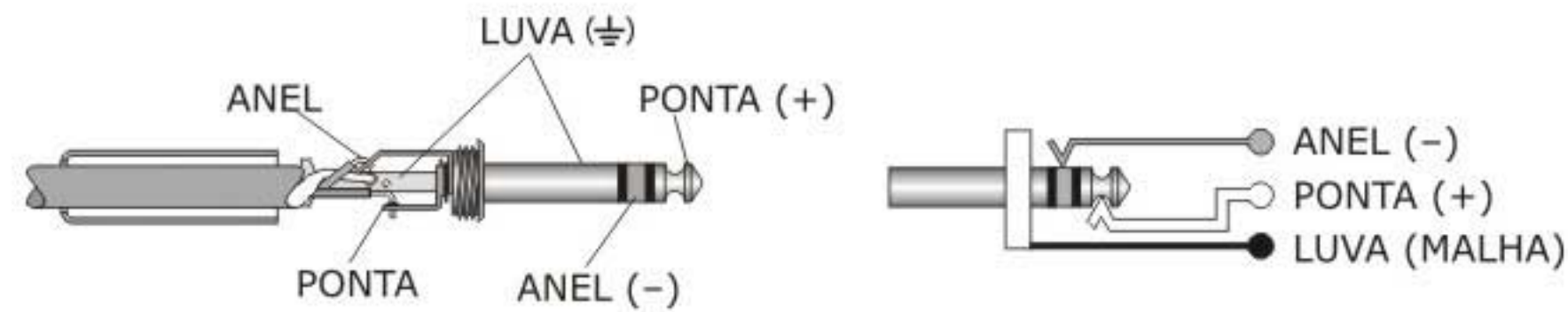
Figura B: Pino 1/4" TRS
